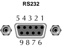
Figure 2-3 RS-232 interface connector
